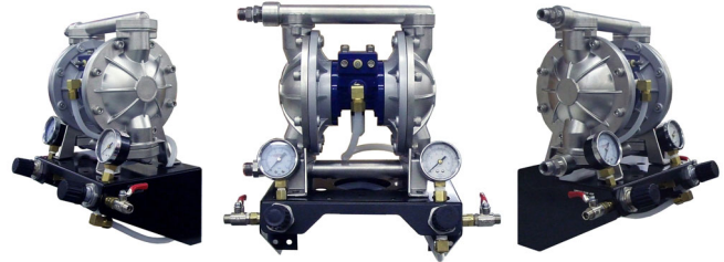
70-1101-5 DOUBLE DIAPHRAGM PUMP WALL MOUNT (5 GALLON SIPHON)
