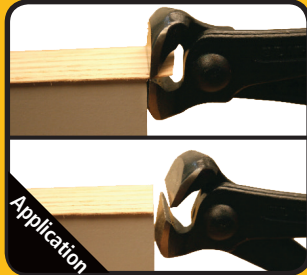
Flush edgbanding with End Nippers
