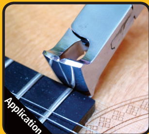
Flush frets with Fret Nippers
